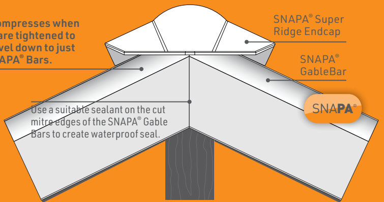
Front elevation detail of the SNAPA® Super Ridge Endcap and SNAPA® Gable Bars
