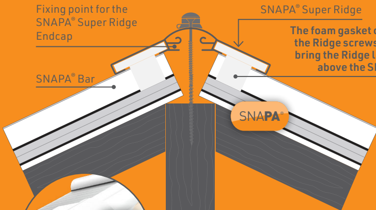
Section detail of the SNAPA® Super Ridge and Foam Gasket
