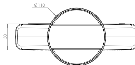
Top Profile
