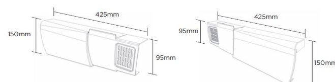
Dry fix verge right hand piece
