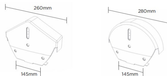
Universal dry fix angled ridge end cap
